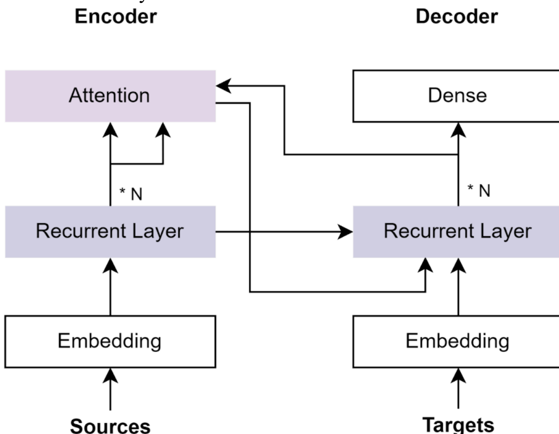
Fig 1 End-to-End Transformer-Based Models in Textual-Based NLP
